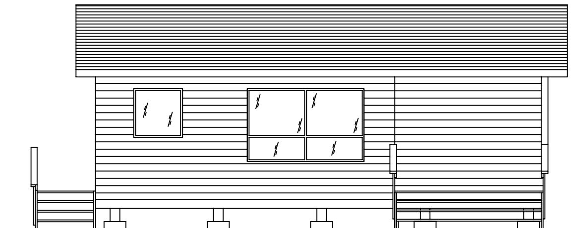
FRONT ELEVATION
